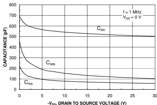
Figure 18. Capacitance Characteristics.
